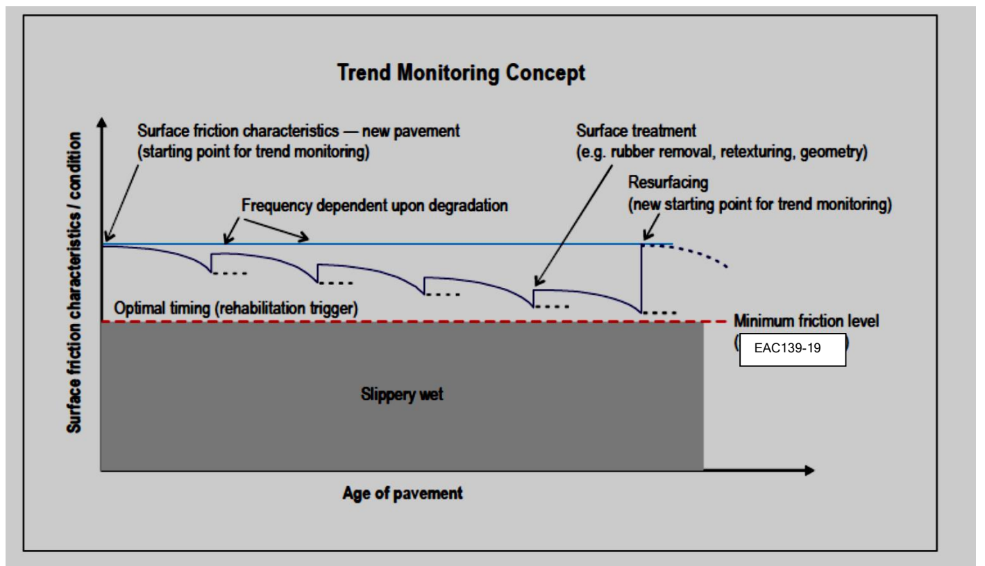
Figure 3-3. Trend monitoring concept (Source: EAC139-19)
