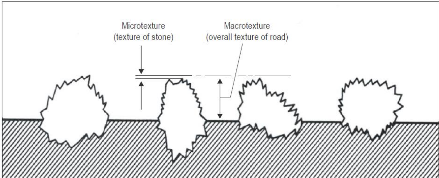
Figure 3-1. Microtexture and macrotexture
